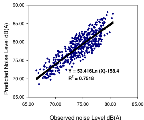
Figure2. Observed Vs. Predicted Noise Level
