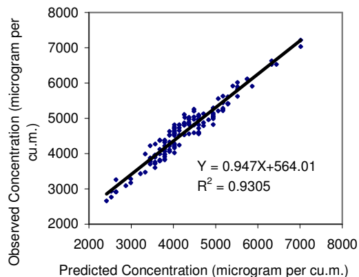
Figure 3. Observed Vs. predicted CO concentrations
